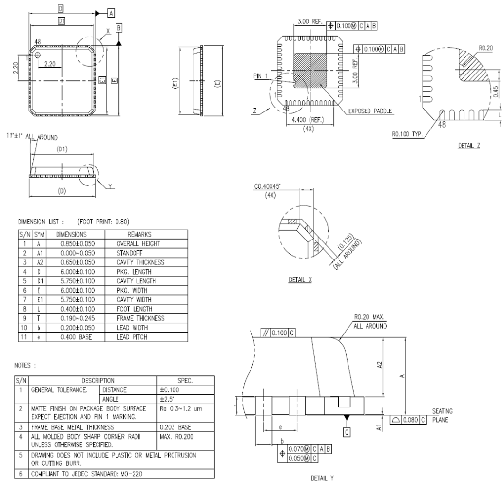
Figure 4-1. Package Illustration
